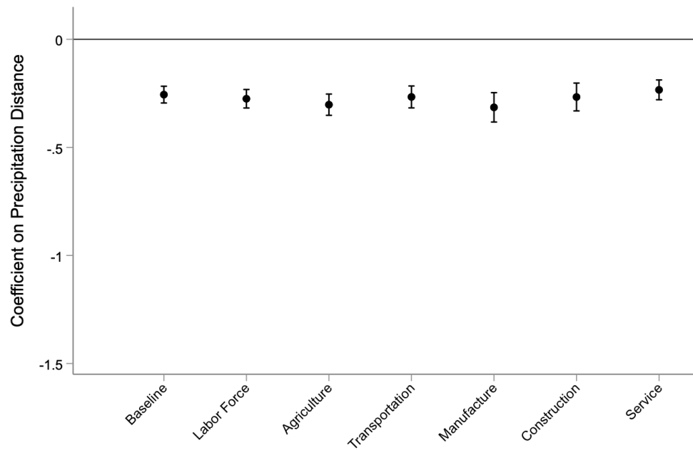
(b) Precipitation
