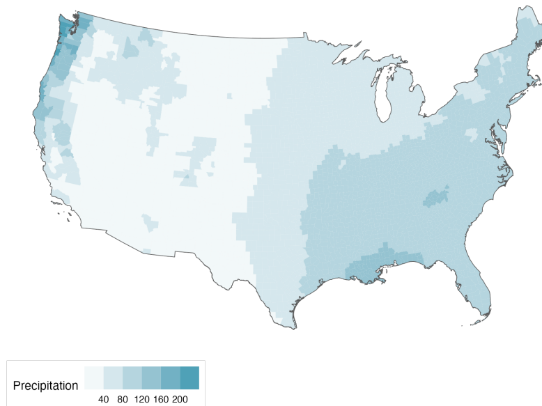
(b) Precipitation
